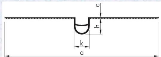
Nitriflex conf. DIN18541 partea 2
