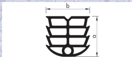
Nitriflex conf. DIN18541 partea 2
